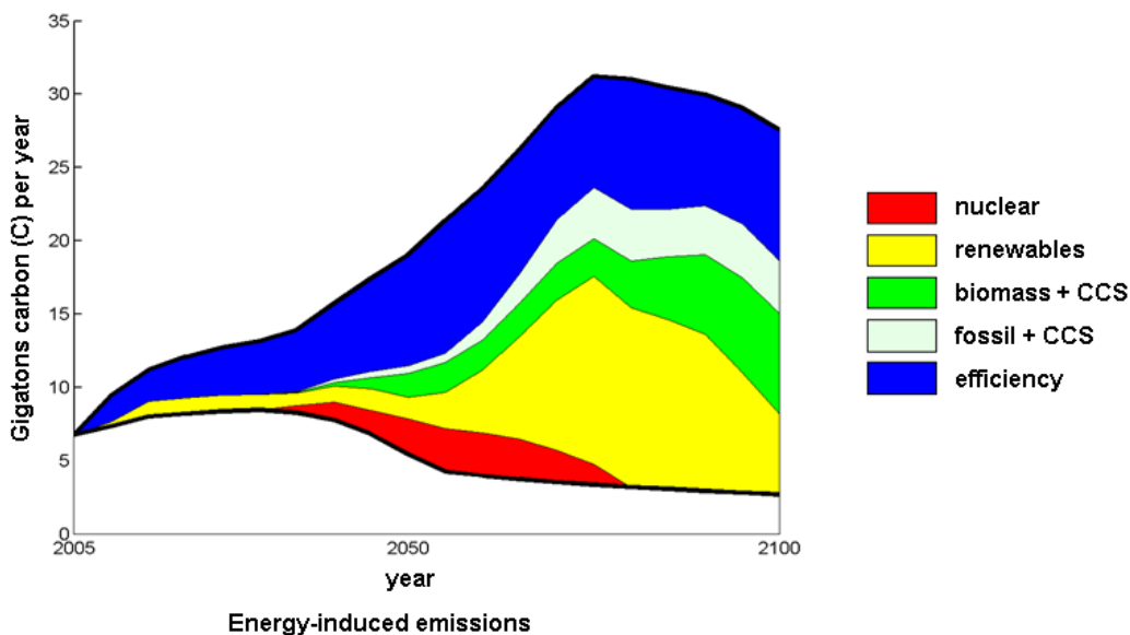
Figure 2: Contribution of mitigation options to global emission reductions in the energy sector for a scenario with cheap fossil fuels. Source: REMIND-G (PIK)
