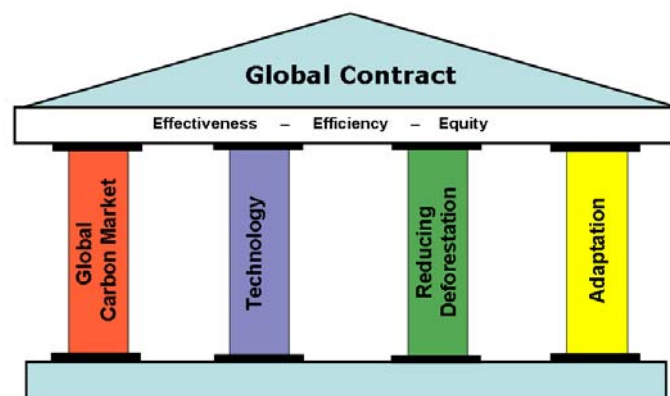
Figure 3: The Global Contract on Climate Change should embrace four major components: a global carbon market, technology, action for reducing deforestation, and adaptation.
